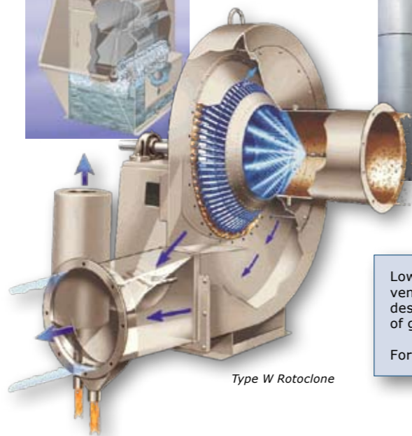
Stainless steel dynamic scrubber
